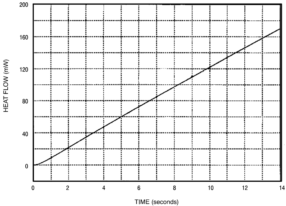
Figure 37. Simulation shows that little heat flows into the environment during the first 14 seconds of operation.
