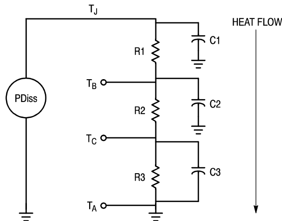
Heat generated in a device’s junction flows from a higher temperature region through each resistor–capacitor pair to a lower temperature region.
