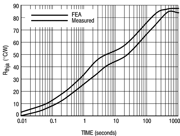
Figure 26. Measured and Modeled R_{thja} for Device 2
