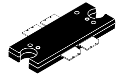
CASE 1484 STYLE 1 PLASTIC (TO-272 WB-4)
