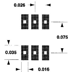
Figure 22. PCB Pad Layout (dimensions in inches).
