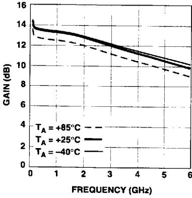
Figure 1. 50 Ω Power Gain vs. Frequency and Temperature.
