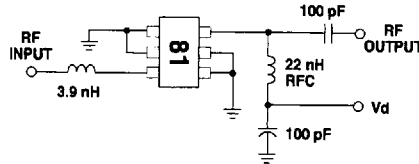
Figure 10. Test Circuit.
