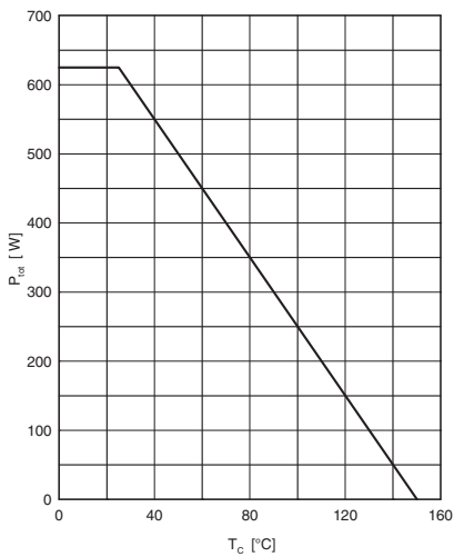
Fig. 1 Power dissipation
